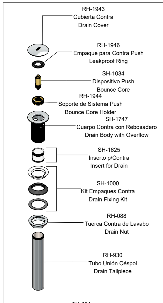
TH-064 Contra de Push para Lavabo con Rebosadero Lavatory Sink Pop-up Drain with Overflow
