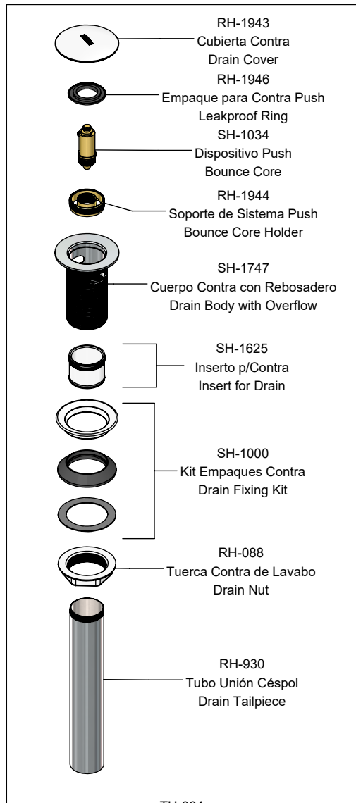
TH-064 Contra de Push para Lavabo con Rebosadero Lavatory Sink Pop-up Drain with Overflow
