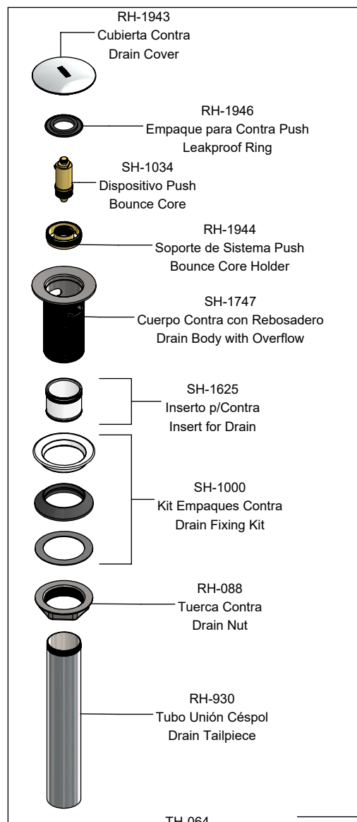
TH-064 Contra de Push para Lavabo con Rebosadero Lavatory Sink Pop-up Drain with Overflow
