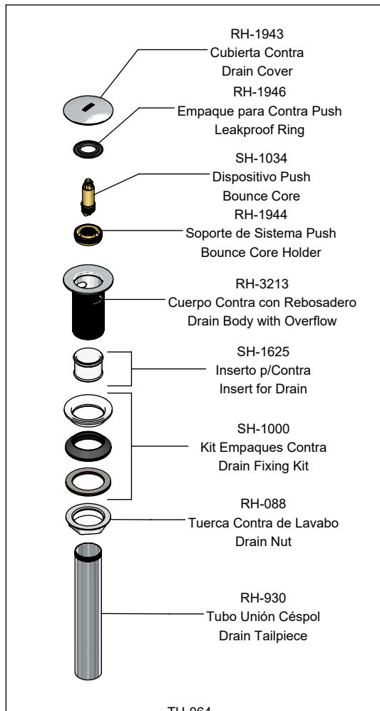
TH-064 Contra de Push para Lavabo con Rebosadero Lavatory Sink Pop-up Drain with Overflow
