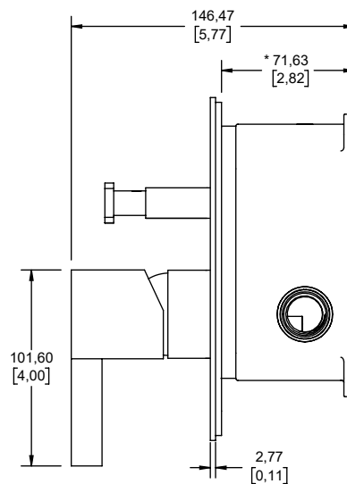
VISTA LATERAL SIDE VIEW
