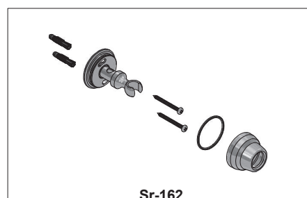
Sr-162 Ancla Chapetón c/ Soporte y Taquetes Escutcheon Anchor w/ Support and Plugs
