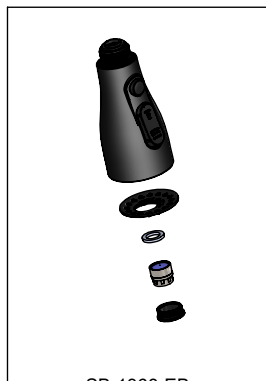
SB-1368-EB Cabezal Head
