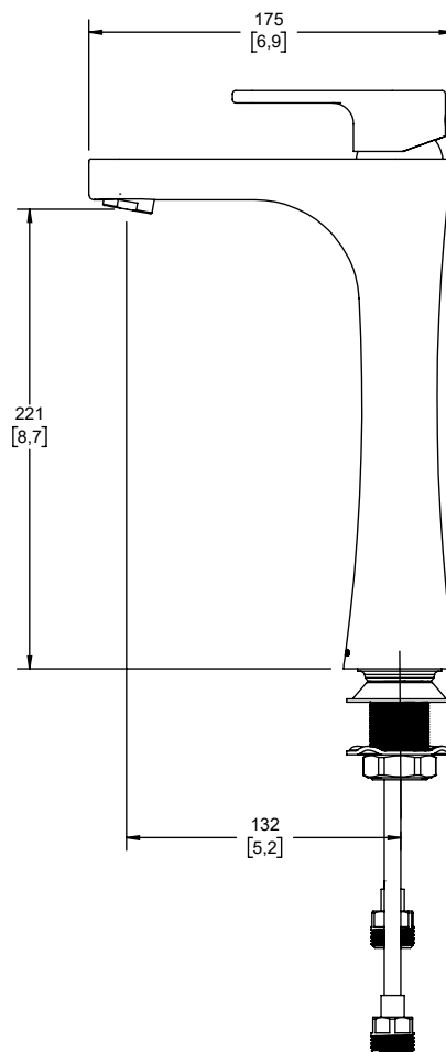
VISTA LATERAL SIDE VIEW
