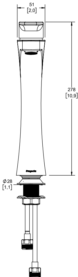
VISTA FRONTAL FRONT VIEW
